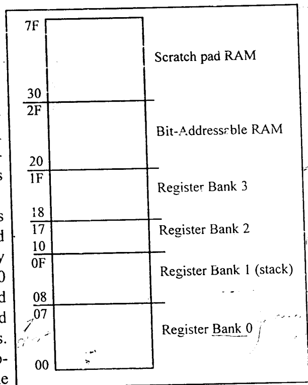
Figure 2-5. RAM Allocation in the 8051
